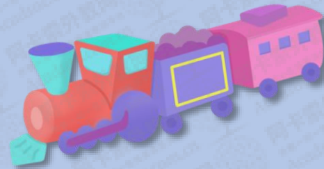
train
