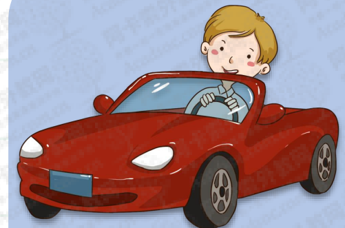
drive
