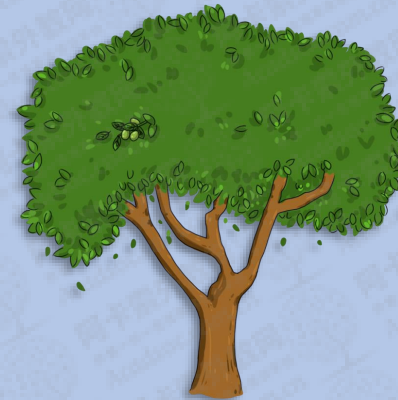
tree
